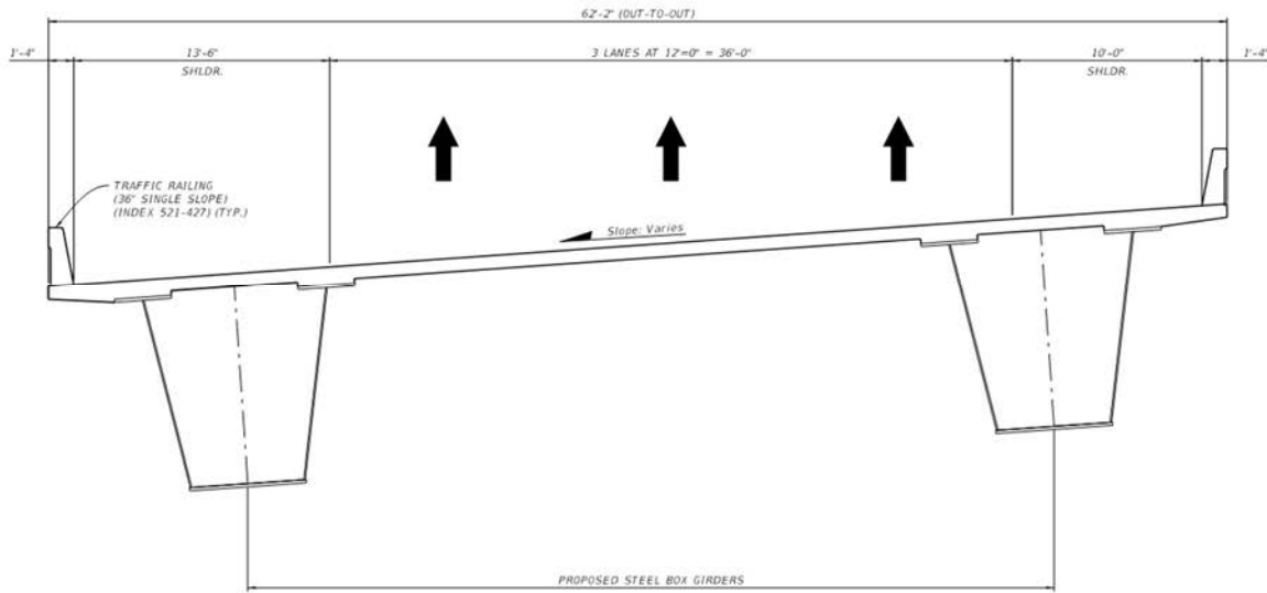
Figure 4-13: Typical Section for Ramp B2
