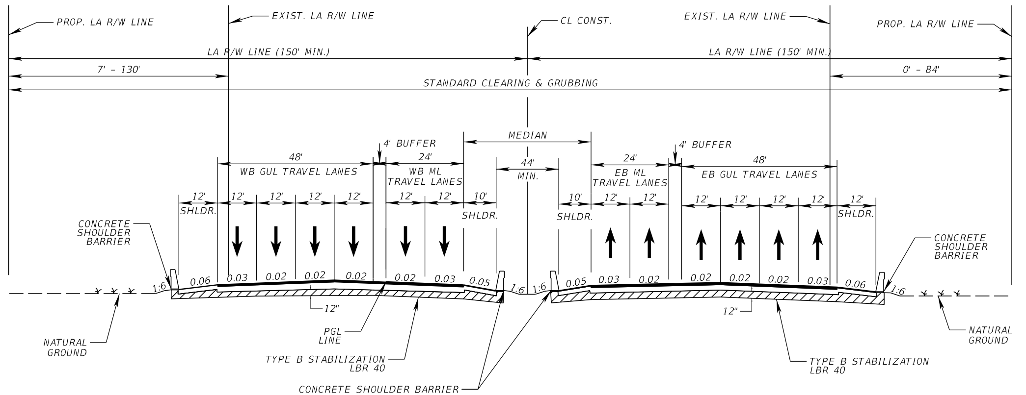
PROPOSED 8-LANE GENERAL USE LANES (GUL) WITH 4-LANE MANAGED LANES (ML) INTERSTATE 4 (BUFFER SEPARATED)
