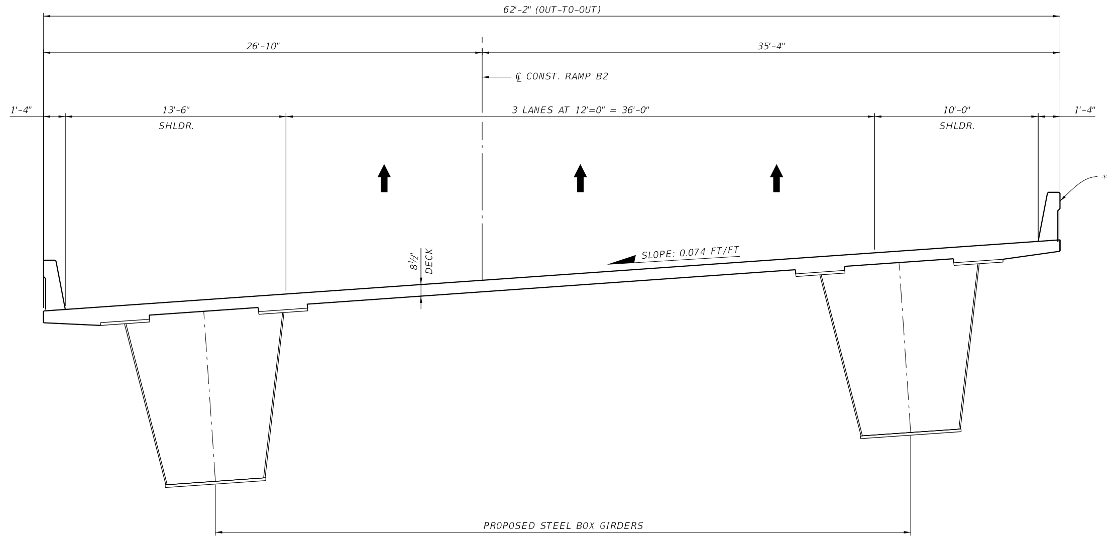
RAMP B2 OVER I-4
