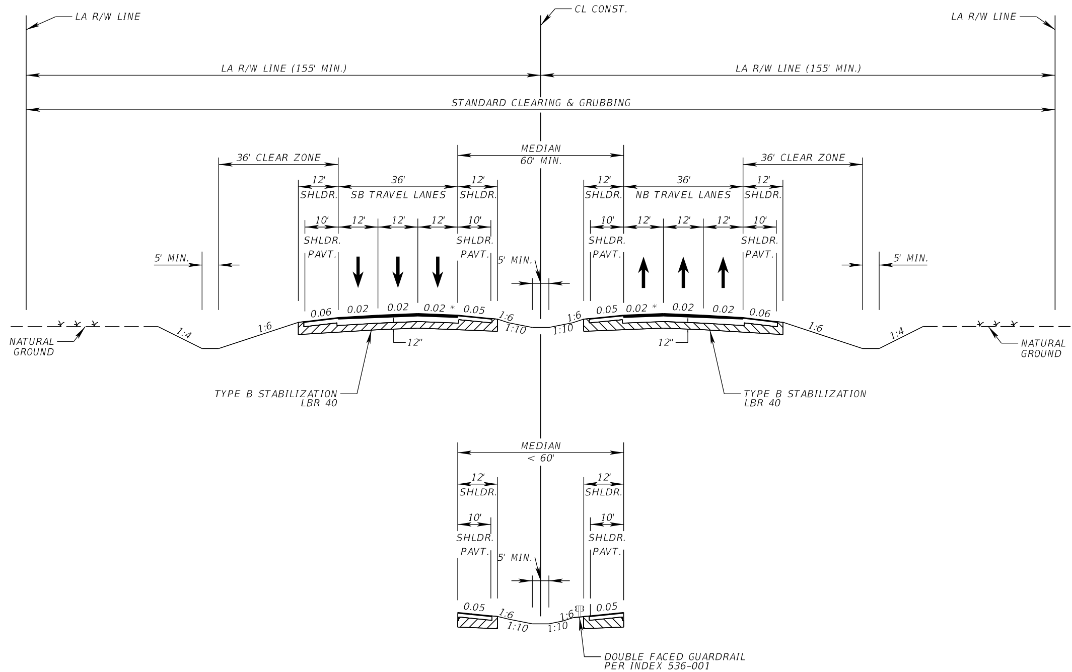
PROPOSED 6-LANE TYPICAL SECTION POINCIANA PARKWAY EXTENSION (SR 538) FROM SR 532 to I-4
