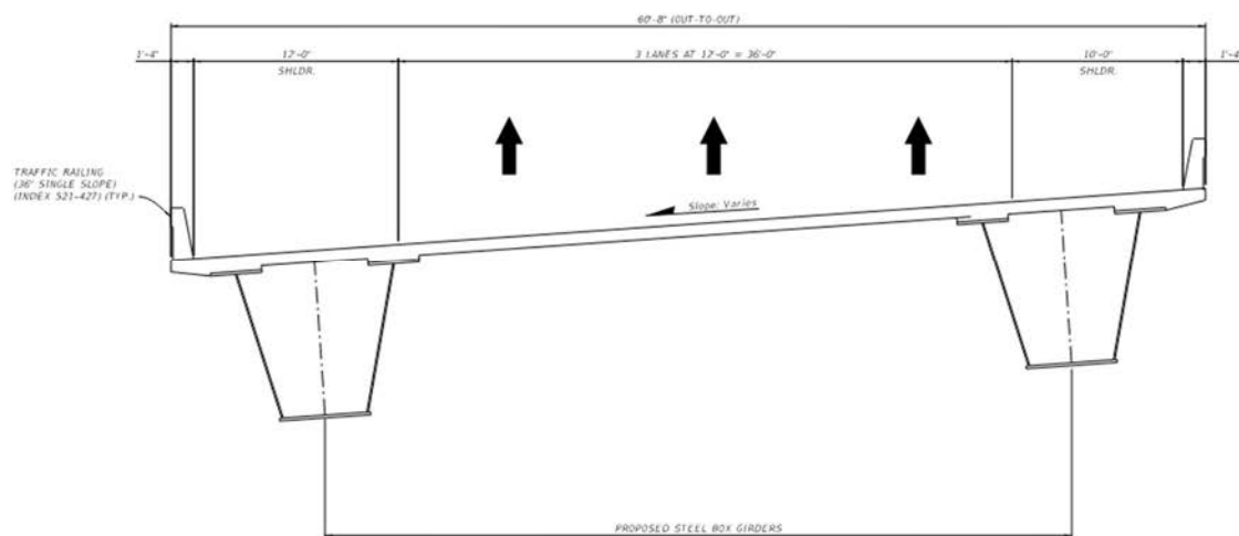
Figure 6-14: Typical Section for Ramp D2 over I-4
