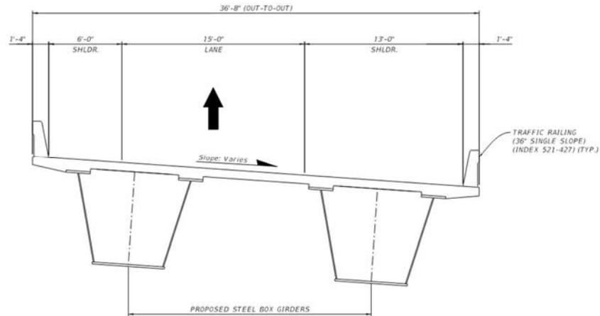
Figure 6-8: Typical Section for Ramp B3
