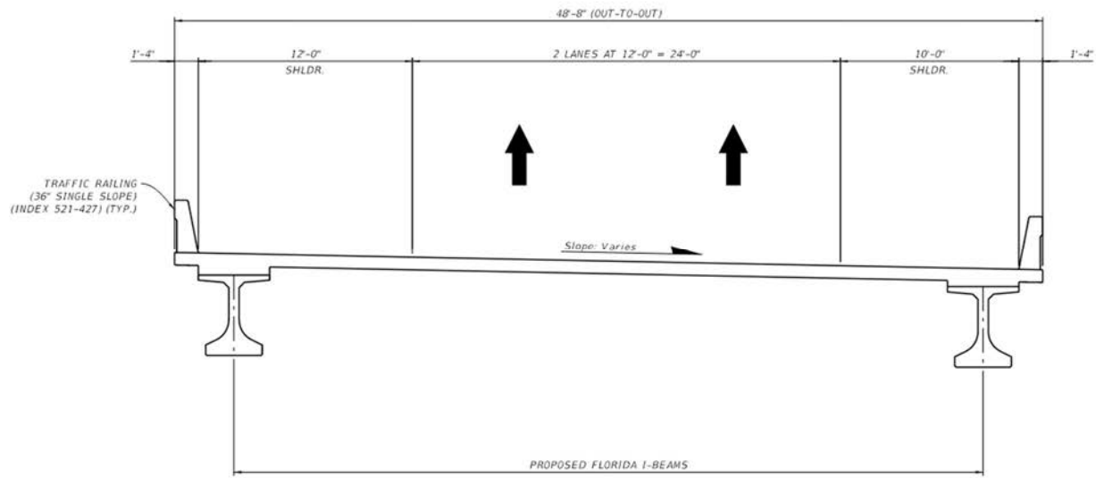
Figure 4-15: Typical Section for Ramp C1
