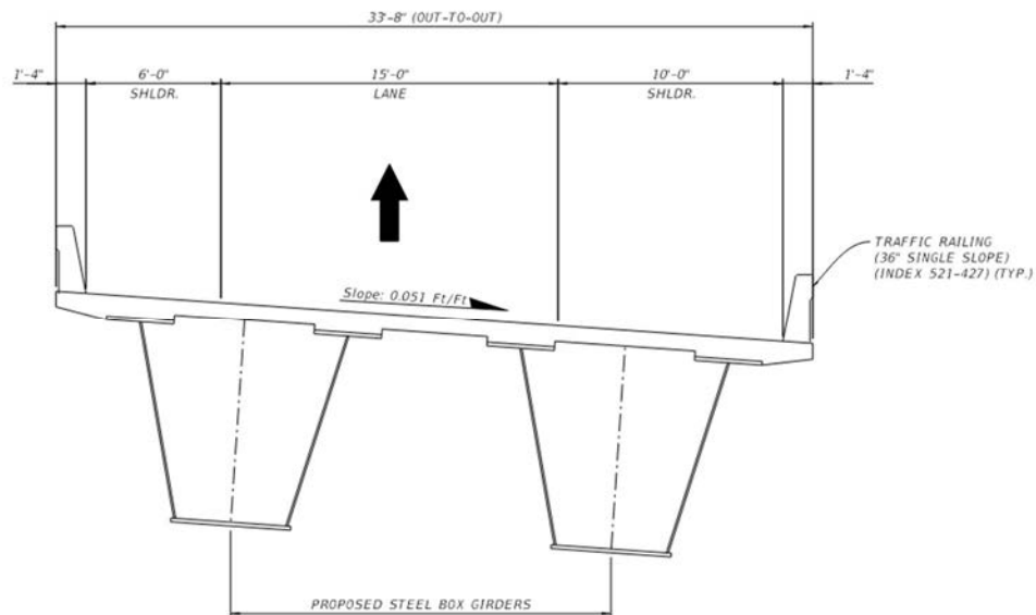
Figure 6-6: Typical Section for Ramp B1
