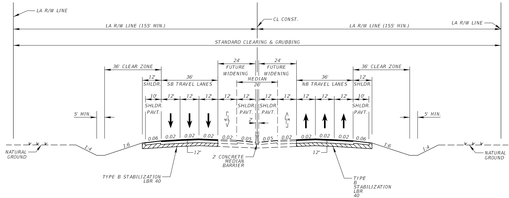
PROPOSED 8-LANE TYPICAL SECTION POINCIANA PARKWAY EXTENSION FUTURE WIDENING (SR 538) FROM SR 532 TO I-4
