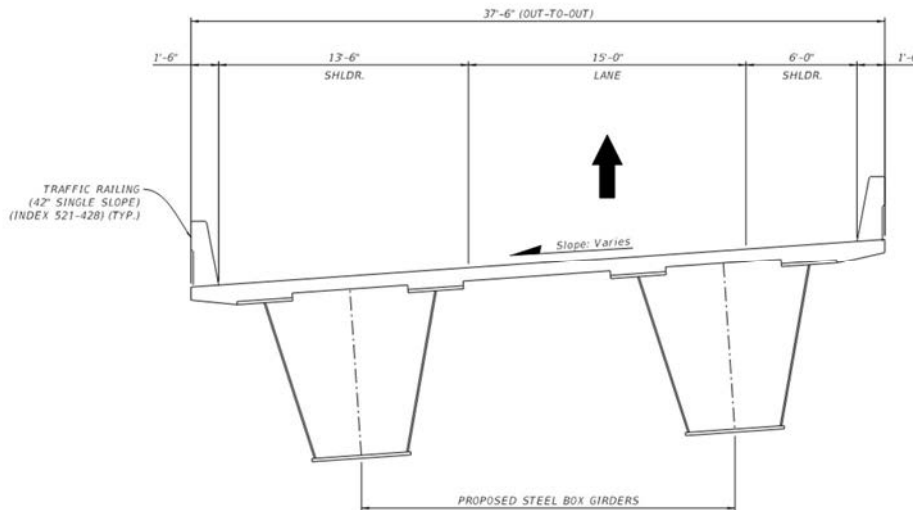
Figure 6-3: Typical Section for Ramp A1
