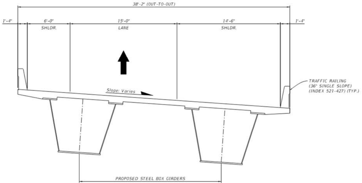
Figure 4-17: Typical Section for Ramp C3
