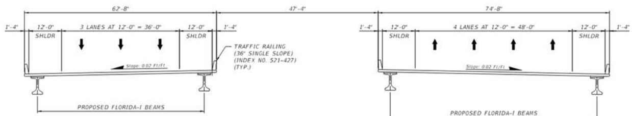
Figure 6-16: Typical Section for Poinciana Parkway (SR 538) over CR 532
