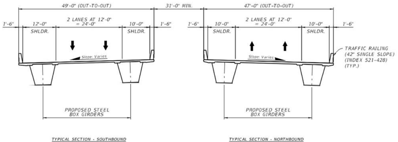
Figure 4-32: Typical Section for Northbound and Southbound Poinciana Parkway (SR 538)
